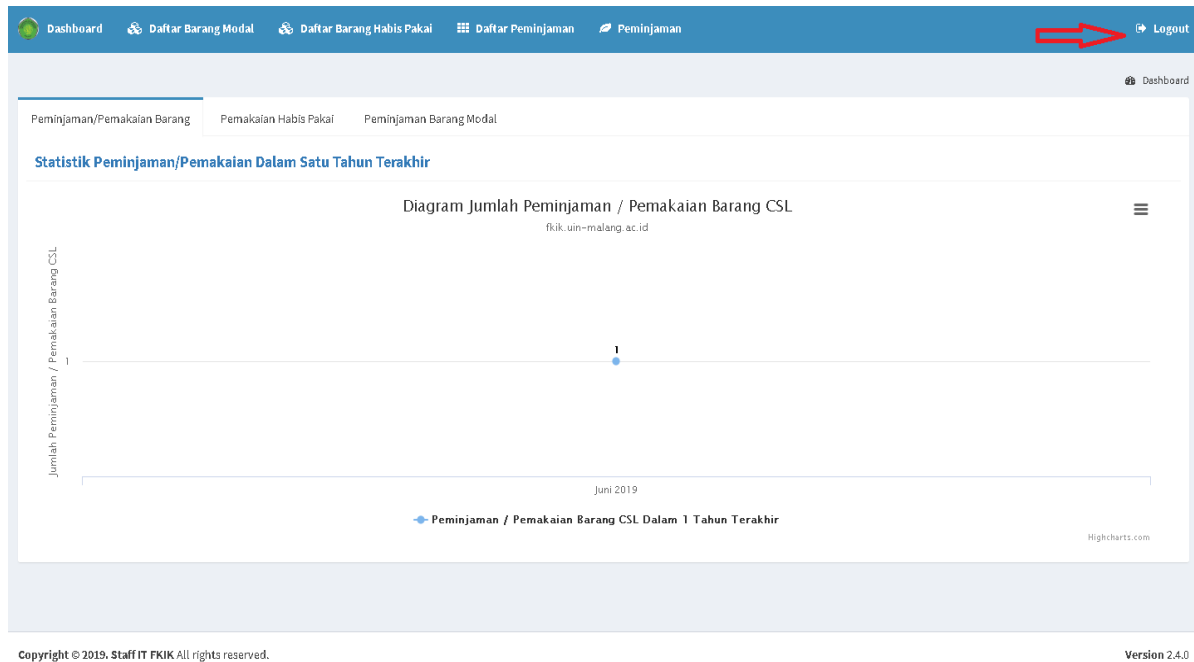
Gambar 10. Log Out
